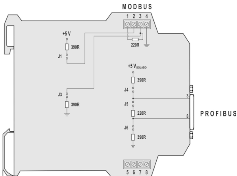
Fig. 4 – Device internal resistors (termination and polarization)
