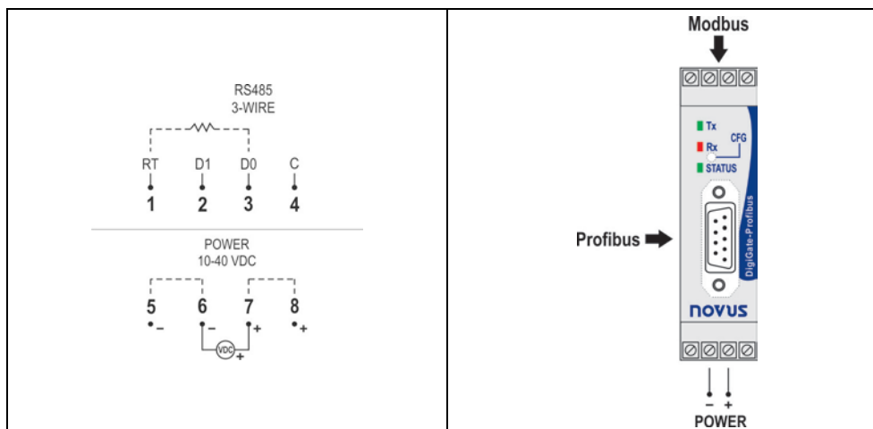
Fig. 2 – Electrical connections
