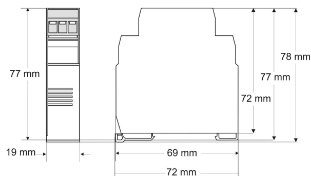
Figure 3 – Dimensions
