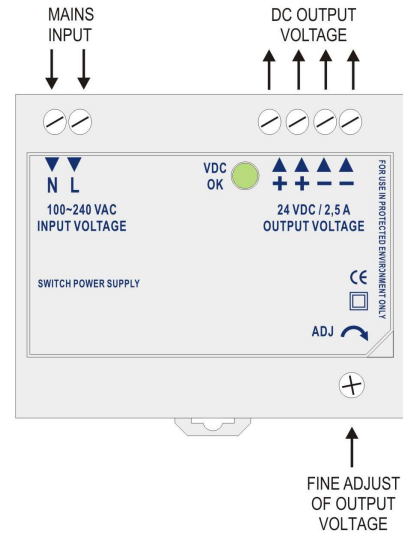
Figure 1 – Electrical connections
