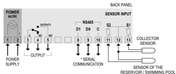
Figure 1 – N321S terminals
