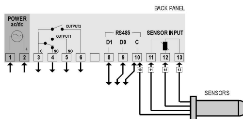
Figure 02 – N322RHT terminals
